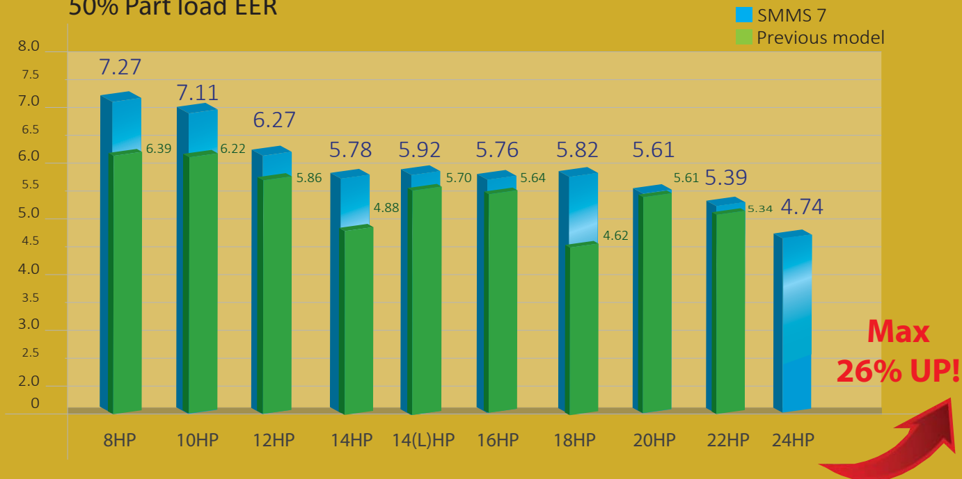
50% Part load EER
