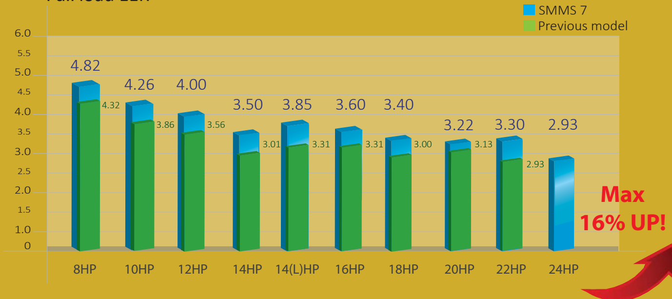
Full load EER
